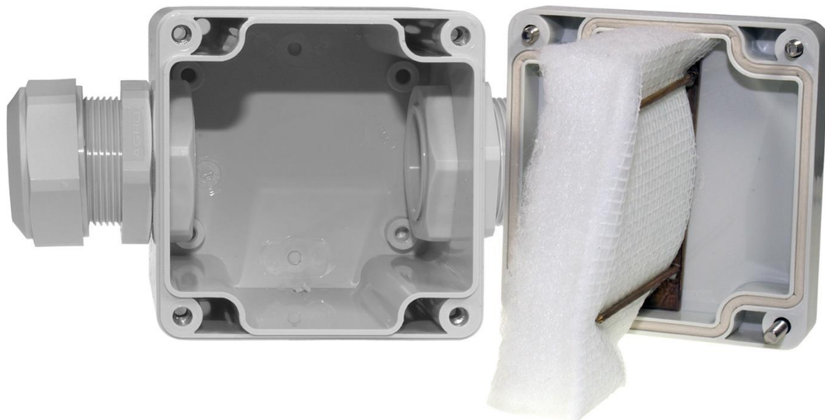
Fig. 1 Filter-box FBS 25 (small) open
