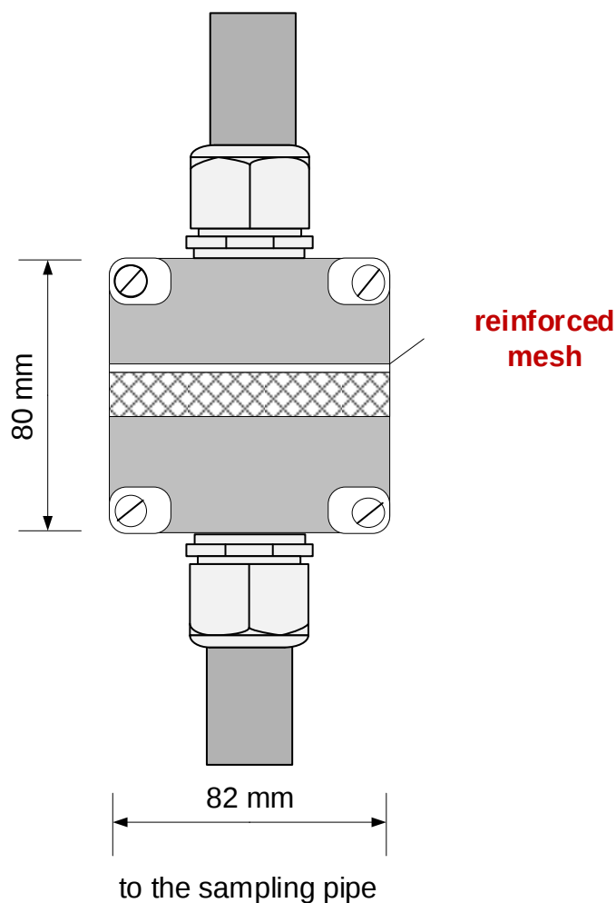
Fig. 4 Mounting orientation filter-box FBS 25 (small)
