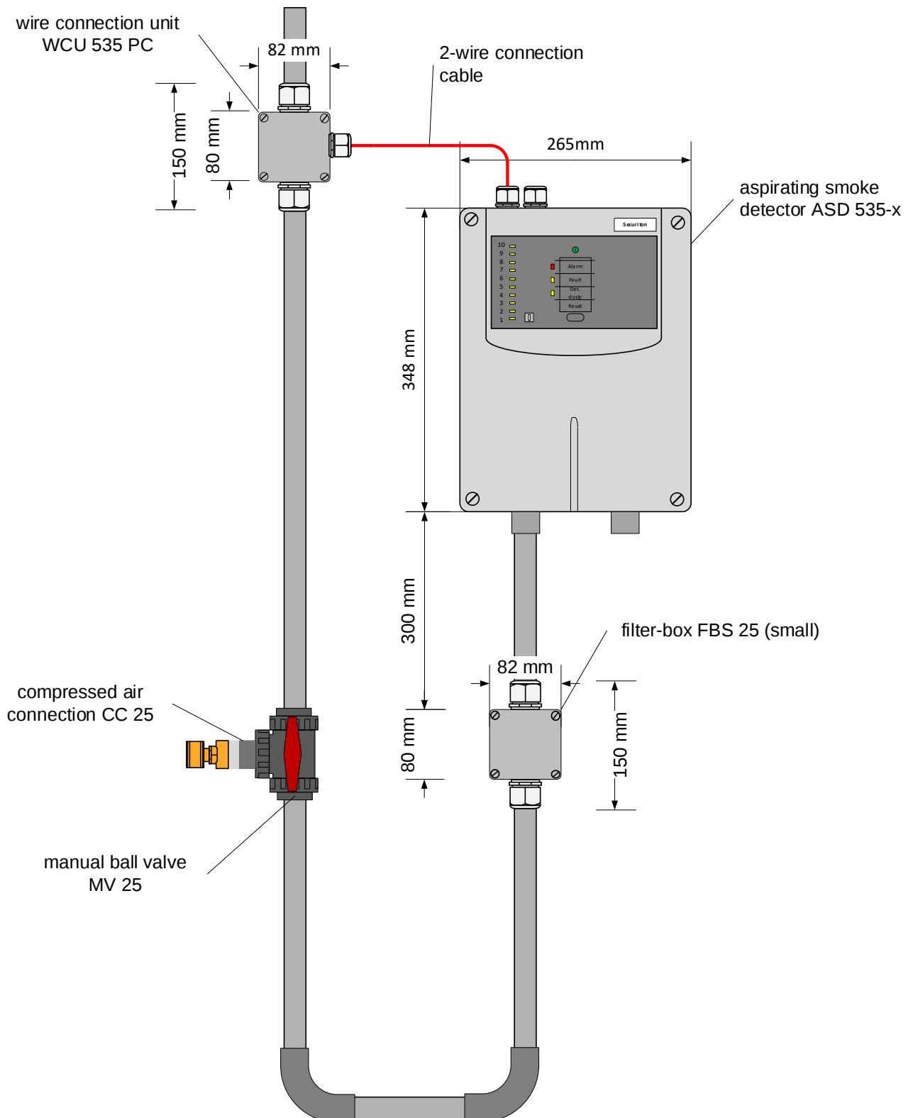
Fig. 2 Standard-Installation for use in deep freeze area with the wiring connection unit WCU 535 PC
